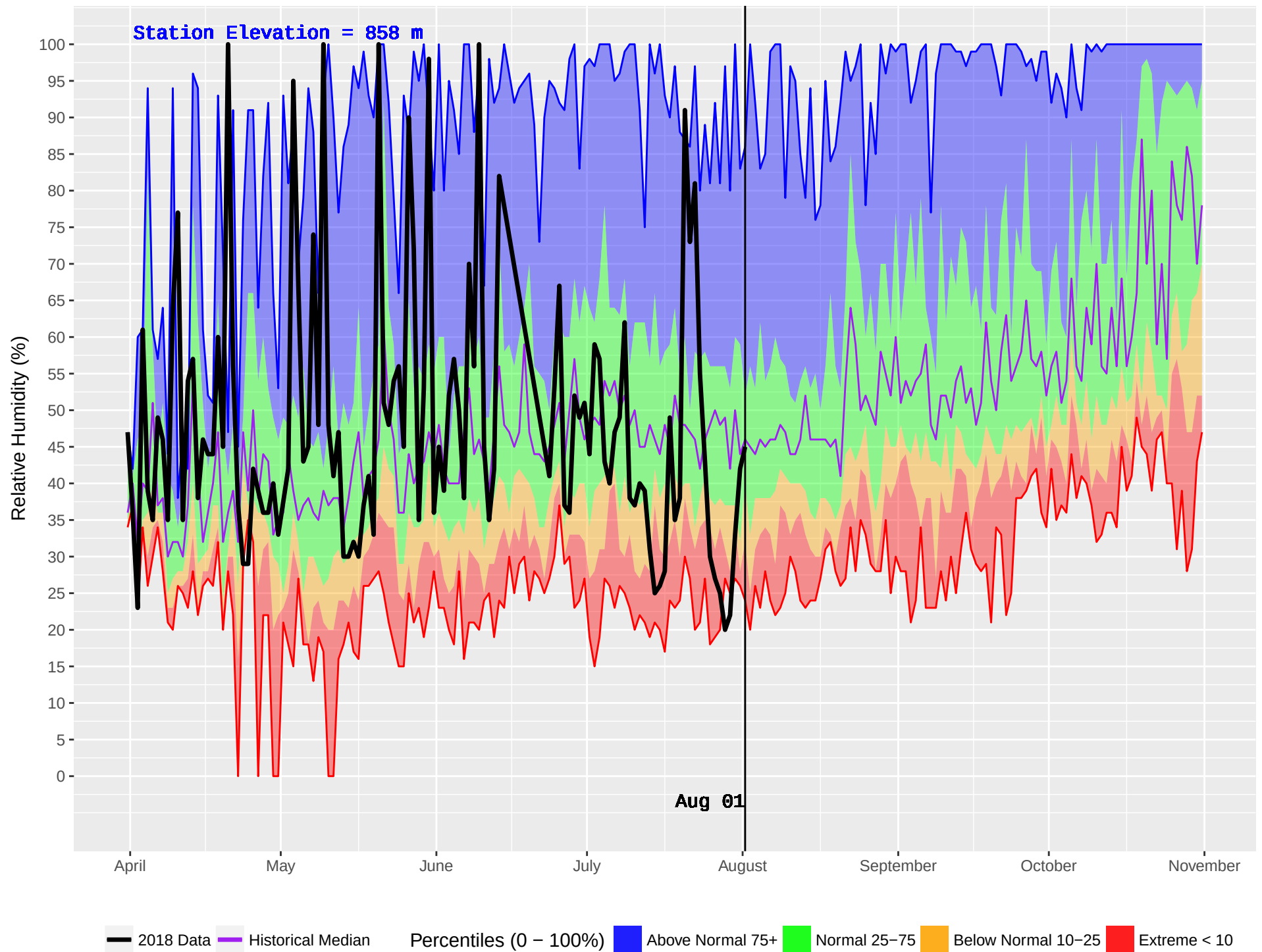
BEDNESTI (175) : Historical (1993–2016) and Current (2018) Daily Relative Humidity
